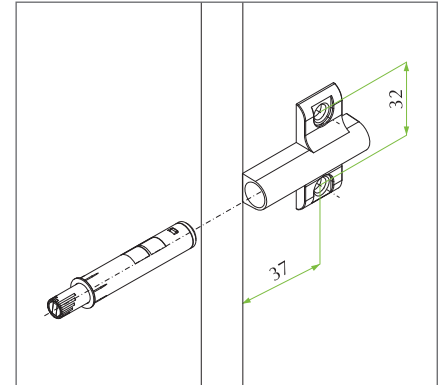
Installation with mounting bracket
