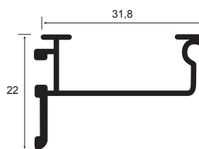
ALUMINIUM HANDLE GRIP SECTION
