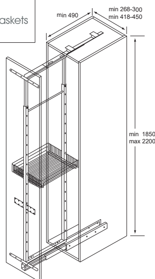
CHROME BASKET for PULLOUT FRAME 6 per Pantry
