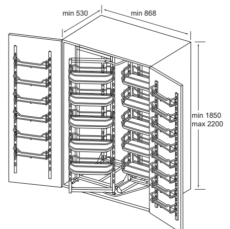
CHROME BASKET for PULLOUT FRAME 24 per Pantry
