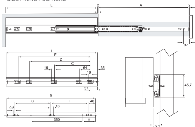
SIDE FIXING POSITIONS
