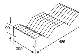
C300 CROCKERY RACK White epoxy coated Suitable for installation in 300mm pot drawer
