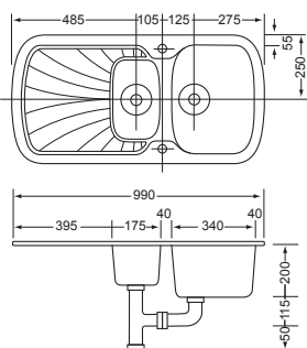
79753 SAPPHIRE 1½ BOWL SINK 990 X 500
