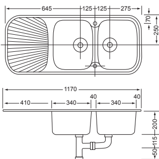
72444 EMERALD DOUBLE BOWL SINK 1170 X 500
