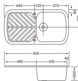
72343 JADE SINGLE BOWL SINK 935 X 500
