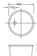
74518 TOPAZ PREP BOWL Ø 460
